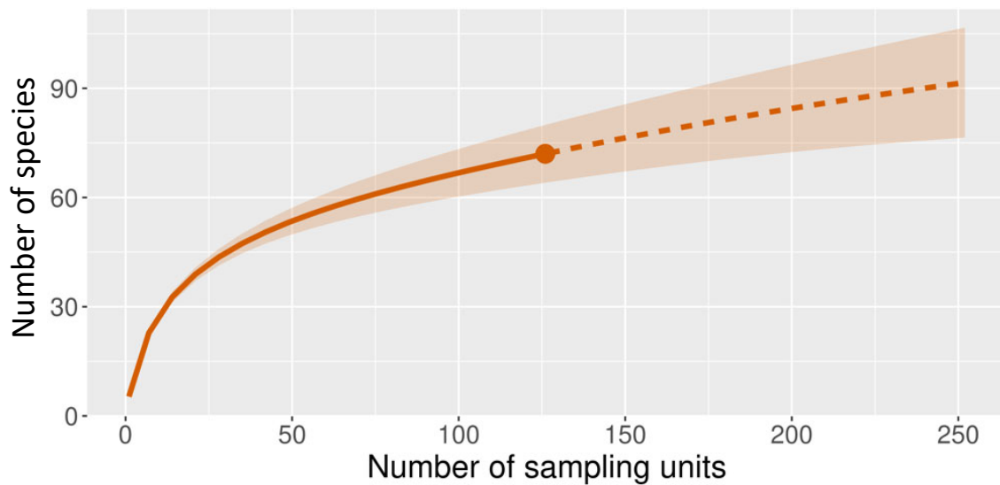
Figure 1. Rarefaction curves for species richness ( q_0 ) calculated with incidence values of the plant species found in four lagoons on the island of Cozumel in Quintana Roo, Mexico.
