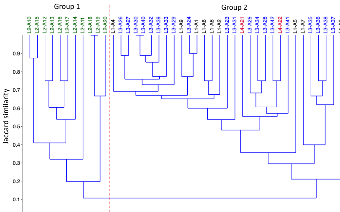
Figure 2. Cluster analysis based on Jaccard index shows floristic similarity between the sampled plots. Dashed red lines differentiate vegetation groups. Color labels in each group show the plots sampled in each lagoon: Black = Lake 1, Green = Lake 2, Blue = Lake 3, and Red = Lake 4.
