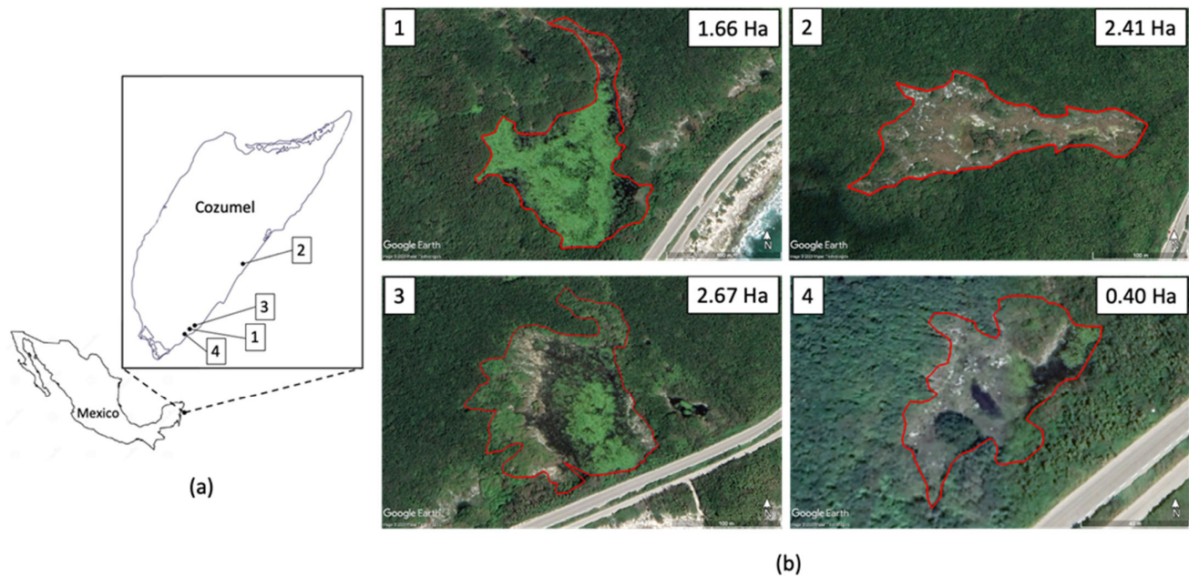
Figure 5. (a) Location of the island of Cozumel in the state of Quintana Roo, southeastern Mexico. The numbers indicate the lagoons studied. (b) Studied lagoons. In each lagoon, the red line shows the surface that is potentially flooded during heavy rainfalls. The flooded surface is shown in the inserted values. Images from Google Earth.
